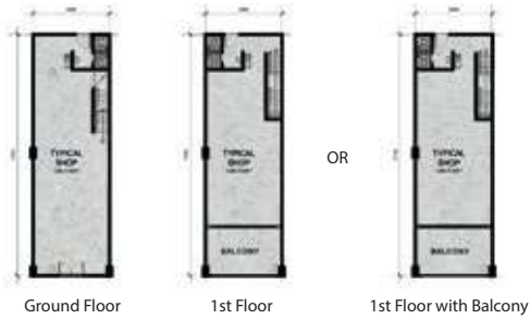
Ground Floor 1st Floor 1st Floor with Balcony
